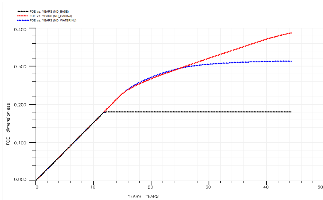
Figure 3 - the recovery factors for water injection and gas injection
